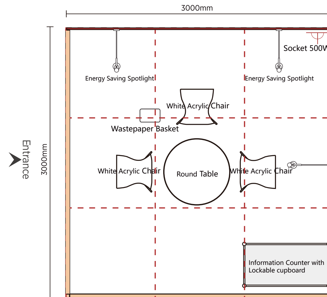
Floorplan
