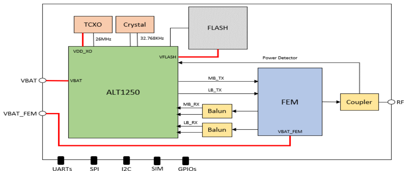
Figure 1.1 Block Diagram
