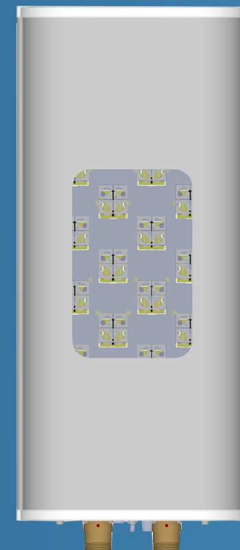
Cable-free Green Antenna S-VPX0407P-E2-C 8T8R TDD 3300-3800MHz 600×270×149mm
