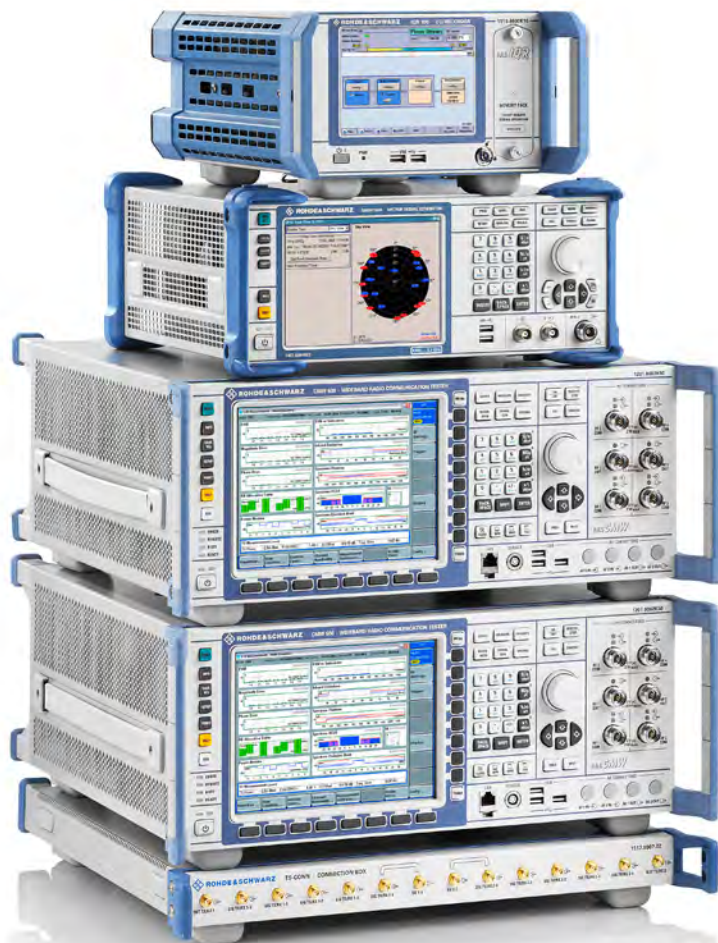
The R&S®TS-LBS advanced test system including carrier acceptance testing
