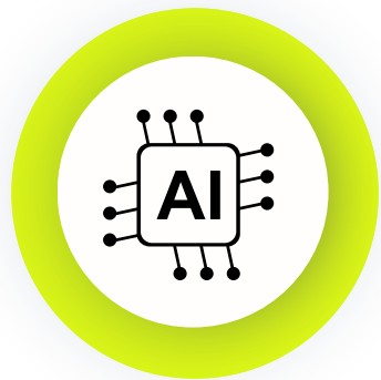
AI Agents
